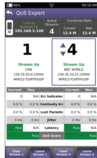
OneExpert CATV IP Video — QoS Expert
