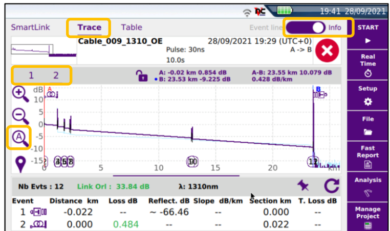
Figure 13: Trace view
